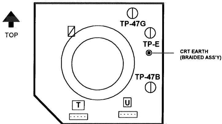
CRT SOCKET PWB (SOLDER SIDE) (Within MAIN PWB)
